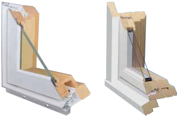
ALUMINUM-CLAD WOOD
